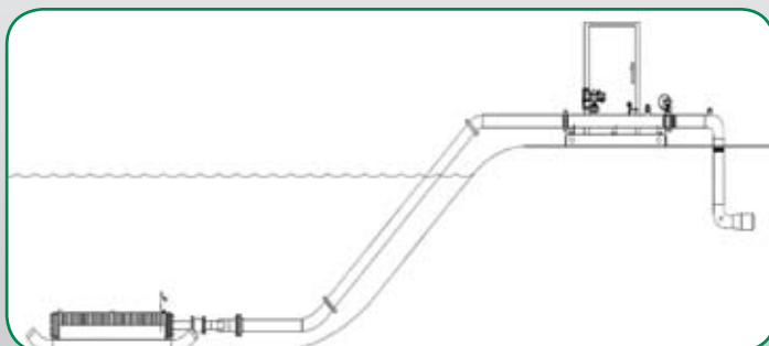
Low profile sled installation
